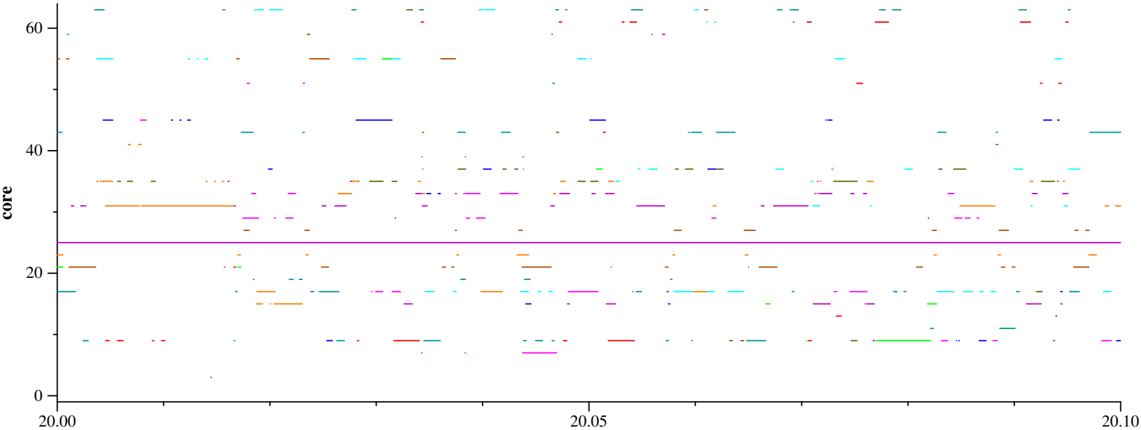
h2 R10 CN dahu-2 5.15.0freq schedutil 1 from 20 upto 20.1, duration: 20.100000, time (seconds)
